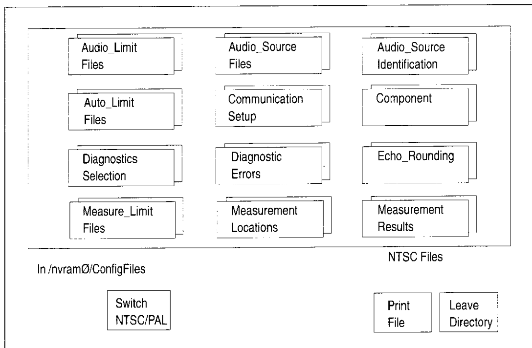
Figure 3-2: Configure Directory
